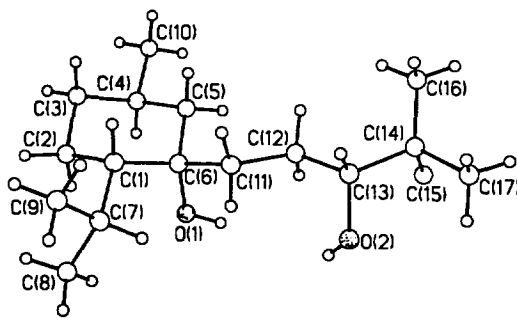
Figure 2. Ball-and-stick representation of the solid state structure 3'b.
