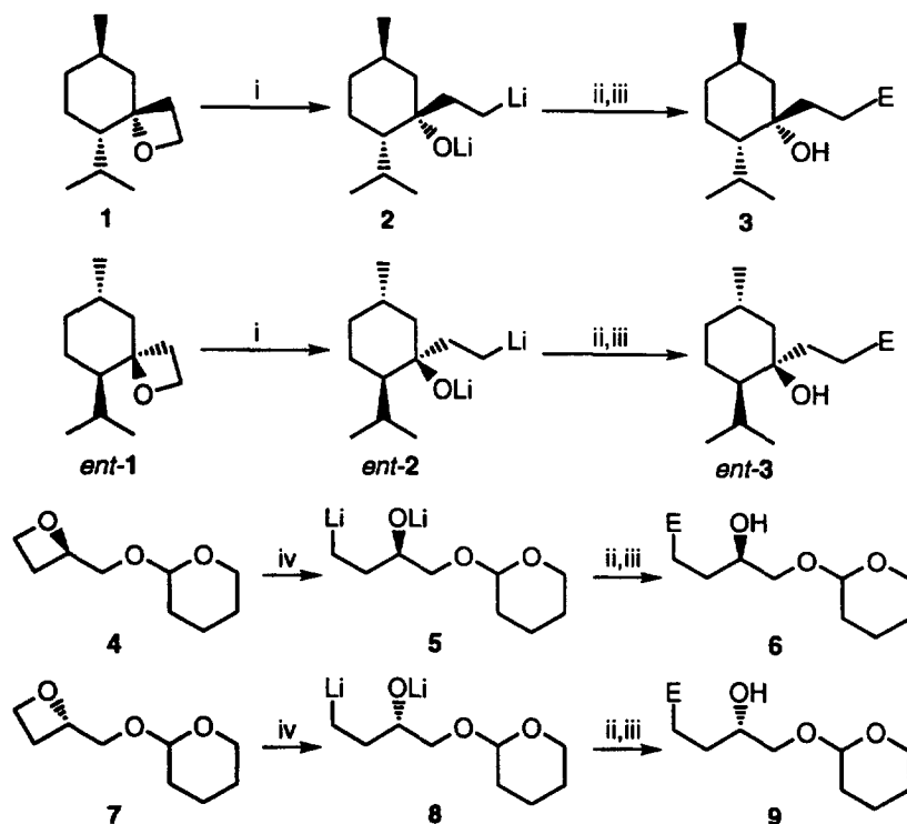
Scheme 1. Reagents and conditions: i, Li, DTBB cat. (5 mol%), THF, 0°C; ii, E + =H 2 O, D 2 O, CO 2 , Bu t CHO, PhCHO, Me 2 CO, (CH 2 ) 5 CO, -78°C; iii, H 2 O, -78 to 20°C; iv, Li, DTBB cat. (5 mol%), THF, -20°C.
