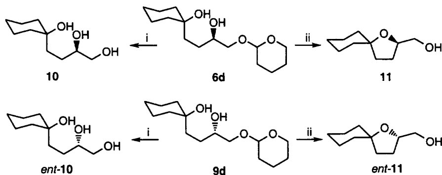
Scheme 2. Reagents and conditions: i, p -TsOH (5 mg), MeOH, 25°C; ii, p -TsOH (15 mg), MeOH, 25°C.
